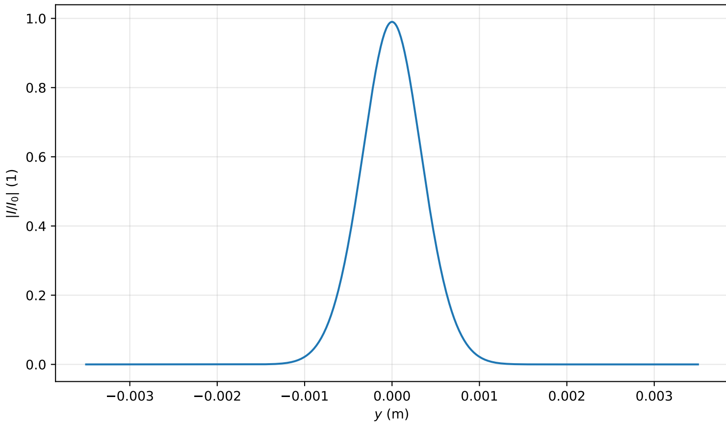
Intensity profile I(x=0, y, z=0.637)/I_0 , P_{in}=0.3P_{cr} , artificial time
